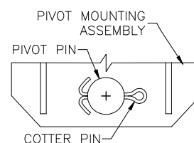
Diagram 2E. Installing cotter pin.
