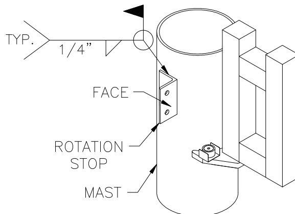
Diagram 7C. Welding rotation stops on the WSJ360.
