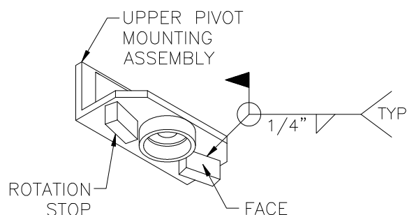
Diagram 7D. Welding rotation stops on the WSJ200.
