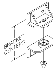
Diagram 2A. Plumbing pivot mounting assemblies.
