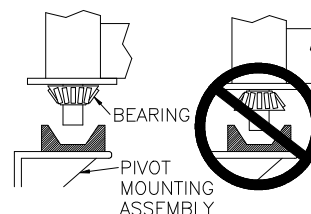
Diagram 2B. Orienting bearing.
