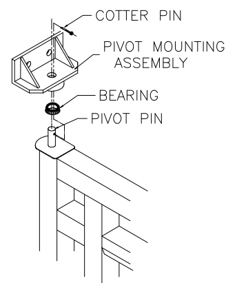
Diagram 2D. Installing upper pivot mounting assembly.
