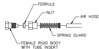
Diagram 11F. Female fitting assembly.
