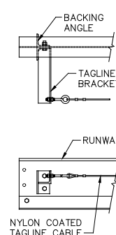
Diagram 9G. Tagline on aluminum runway.
