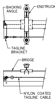
Diagram 9F. Tagline on non-coped aluminum bridge.
